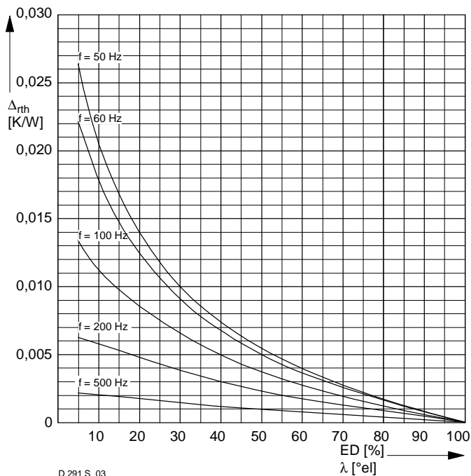
Fig. 3 \Delta_{rth} = f(ED, \text{frequency})
