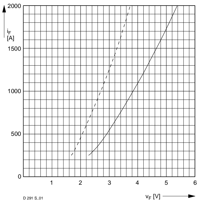
Fig. 1 On-state characteristics i_F = f(v_F) t_{vj} = 125^\circ\text{C}
