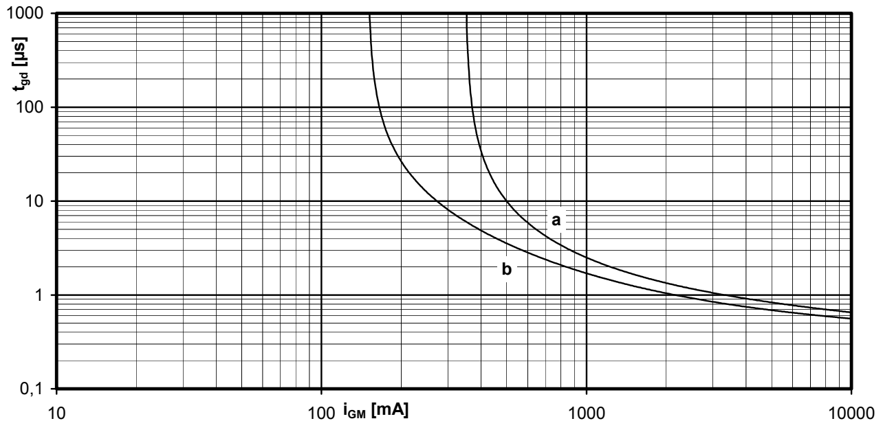
Zündverzug / Gate controlled delay time t_{gd} = f(i_G)
