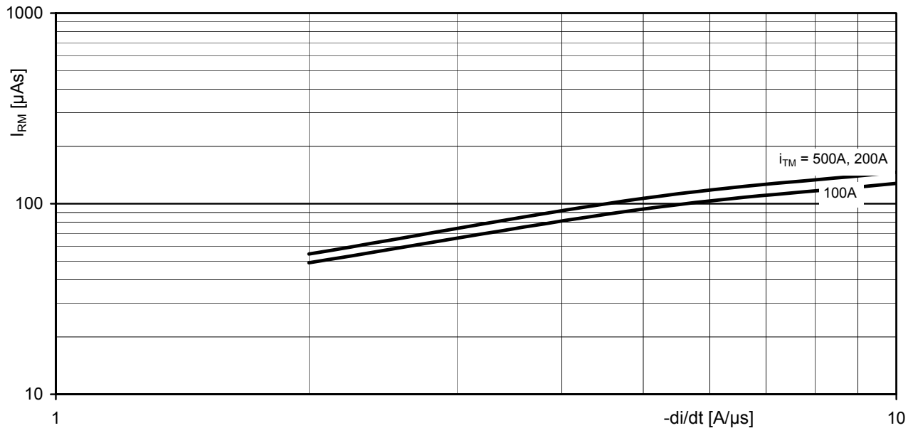
Rückstromspitze / Peak recovery current I_{RM} = f(di/dt)
