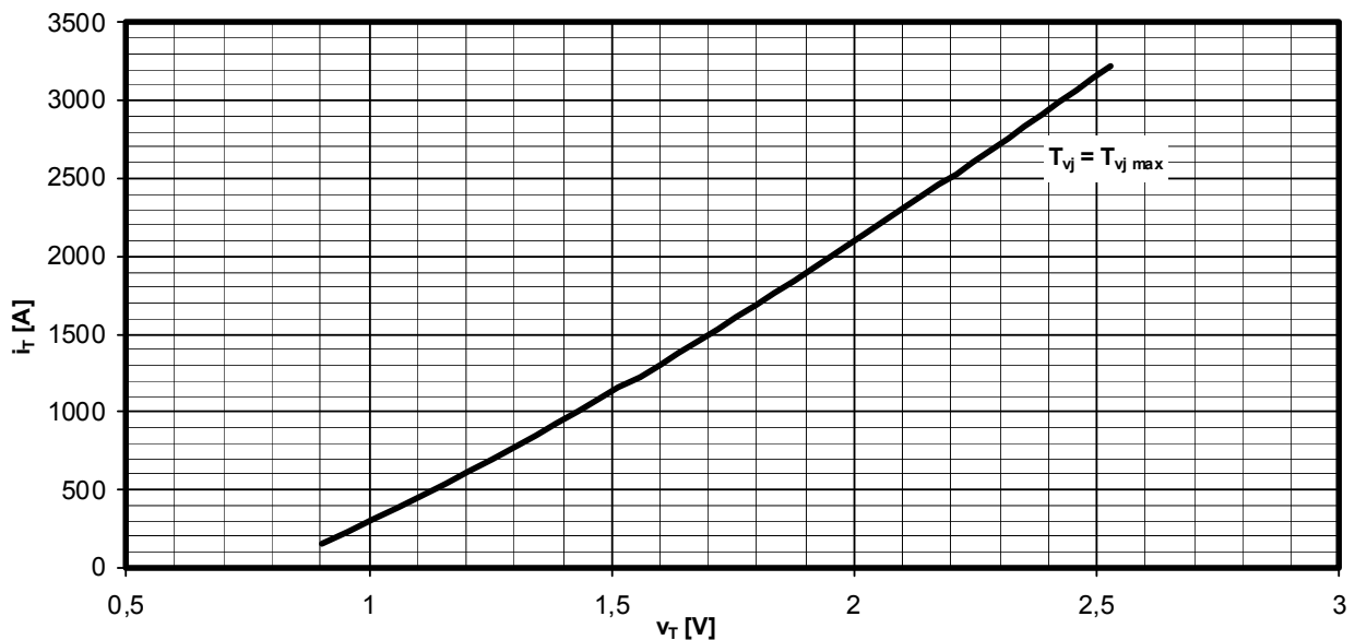
Grenzdurchlasskennlinie / Limiting on-state characteristic i_T = f(v_T)
