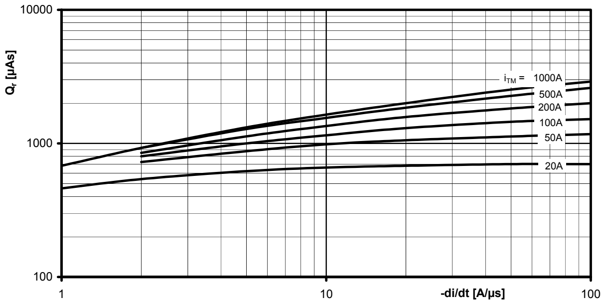
Sperrverzögerungsladung / Recovered charge Q_r = f(di/dt)
