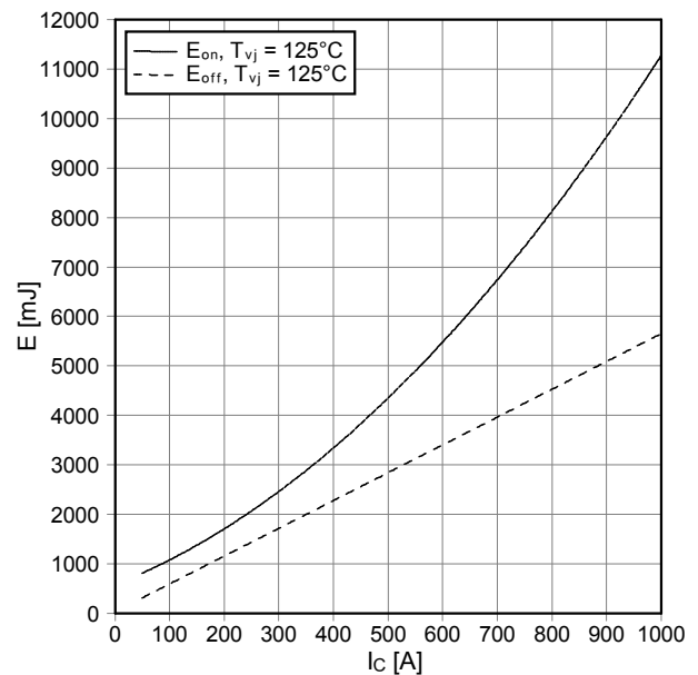
Schaltverluste IGBT-Wechselr. (typisch) switching losses IGBT-inverter (typical) E_{on} = f(I_c) , E_{off} = f(I_c) V_{GE} = \pm 15\text{ V} , R_{Gon} = 1.5\ \Omega , R_{Goff} = 10\ \Omega , V_{CE} = 3600\text{ V}
