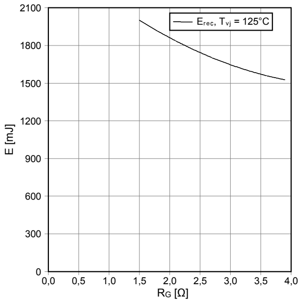
Schaltverluste Diode-Brems-Chopper switching losses Diode-brake-chopper E_{rec} = f(R_G) I_F = 500\text{ A}, V_{CE} = 3600\text{ V}
