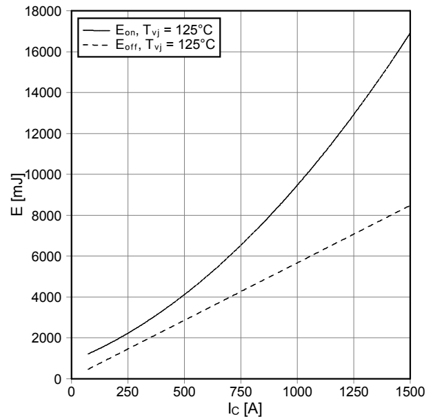
Schaltverluste IGBT-Wechselr. (typisch) switching losses IGBT-inverter (typical) E_{on} = f(I_c) , E_{off} = f(I_c) V_{GE} = \pm 15\text{ V} , R_{Gon} = 1\ \Omega , R_{Goff} = 6.8\ \Omega , V_{CE} = 3600\text{ V}
