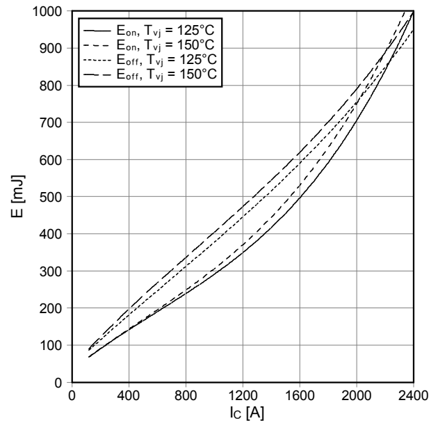
Schaltverluste IGBT-Wechselr. (typisch) switching losses IGBT-inverter (typical) E_{on} = f(I_c) , E_{off} = f(I_c) V_{GE} = \pm 15\text{ V} , R_{Gon} = 0.22\ \Omega , R_{Goff} = 0.9\ \Omega , V_{CE} = 900\text{ V}
