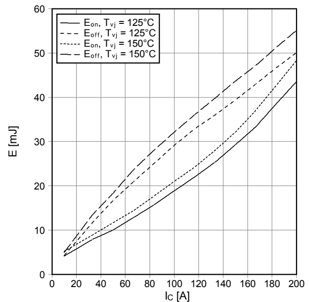
Schaltverluste IGBT-Wechselr. (typisch) switching losses IGBT-inverter (typical) E_{on} = f(I_c) , E_{off} = f(I_c) V_{GE} = \pm 15\text{ V} , R_{Gon} = 0.91\ \Omega , R_{Goff} = 0.91\ \Omega , V_{CE} = 900\text{ V}
