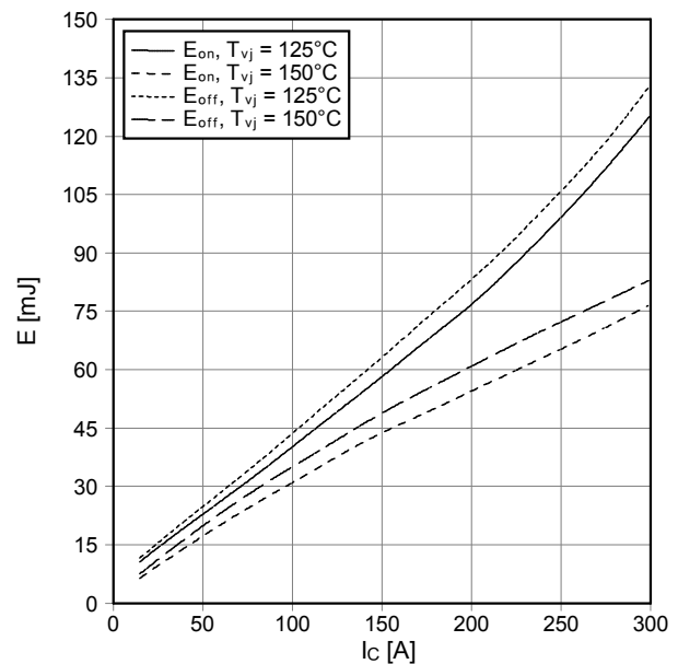
Schaltverluste IGBT-Wechselr. (typisch) switching losses IGBT-inverter (typical) E_{on} = f(I_c) , E_{off} = f(I_c) V_{GE} = \pm 15\text{ V} , R_{Gon} = 4.8\ \Omega , R_{Goff} = 4.8\ \Omega , V_{CE} = 900\text{ V}
