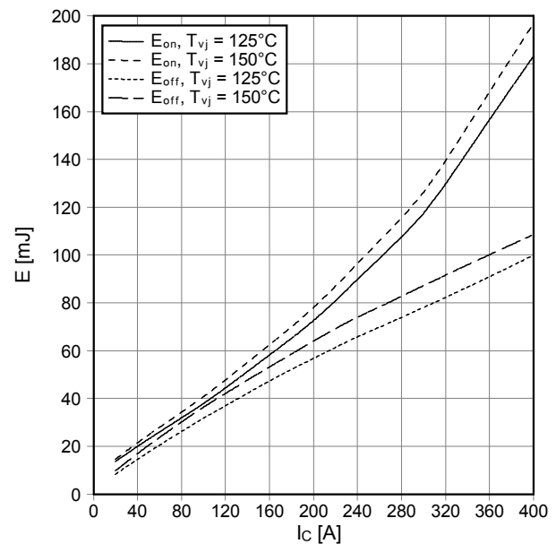
Schaltverluste IGBT-Wechselr. (typisch) switching losses IGBT-inverter (typical) E_{on} = f(I_c) , E_{off} = f(I_c) V_{GE} = \pm 15\text{ V} , R_{Gon} = 3.6\ \Omega , R_{Goff} = 3.6\ \Omega , V_{CE} = 900\text{ V}
