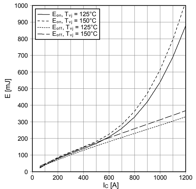
Schaltverluste IGBT-Wechselr. (typisch) switching losses IGBT-inverter (typical) E_{on} = f(I_c) , E_{off} = f(I_c) V_{GE} = \pm 15\text{ V} , R_{Gon} = 1\ \Omega , R_{Goff} = 1\ \Omega , V_{CE} = 900\text{ V}
