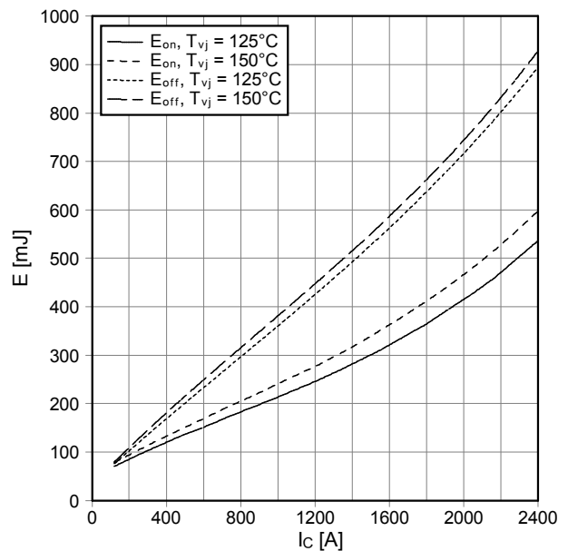
Schaltverluste IGBT-Wechselr. (typisch) switching losses IGBT-inverter (typical) E_{on} = f(I_c) , E_{off} = f(I_c) V_{GE} = \pm 15\text{ V} , R_{Gon} = 0.2\ \Omega , R_{Goff} = 0.8\ \Omega , V_{CE} = 900\text{ V}
