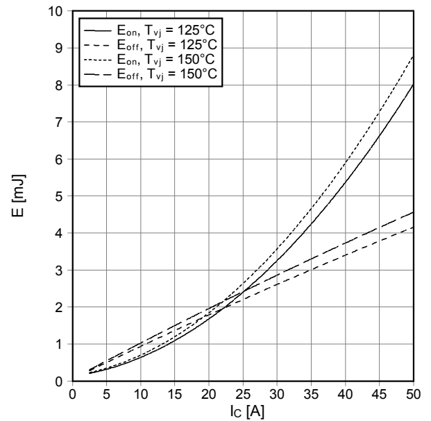
Schaltverluste IGBT-Wechselr. (typisch) switching losses IGBT-inverter (typical) E_{on} = f(I_c) , E_{off} = f(I_c) V_{GE} = \pm 15\text{ V} , R_{Gon} = 18\ \Omega , R_{Goff} = 18\ \Omega , V_{CE} = 600\text{ V}
