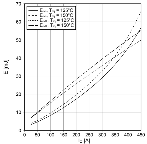
Schaltverluste IGBT-Wechselr. (typisch) switching losses IGBT-inverter (typical) E_{on} = f(I_c) , E_{off} = f(I_c) V_{GE} = \pm 15\text{ V} , R_{Gon} = 0.75\ \Omega , R_{Goff} = 0.75\ \Omega , V_{CE} = 600\text{ V}
