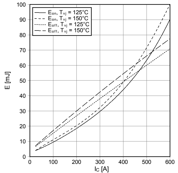
Schaltverluste IGBT-Wechselr. (typisch) switching losses IGBT-inverter (typical) E_{on} = f(I_c) , E_{off} = f(I_c) V_{GE} = \pm 15\text{ V} , R_{Gon} = 0.75\ \Omega , R_{Goff} = 0.75\ \Omega , V_{CE} = 600\text{ V}
