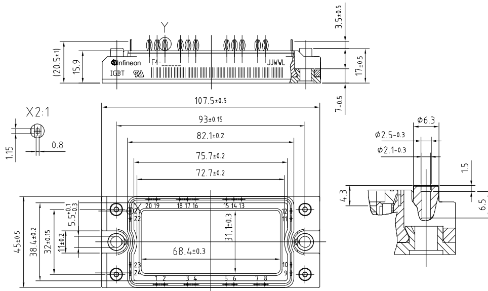
PCB hole pattern
