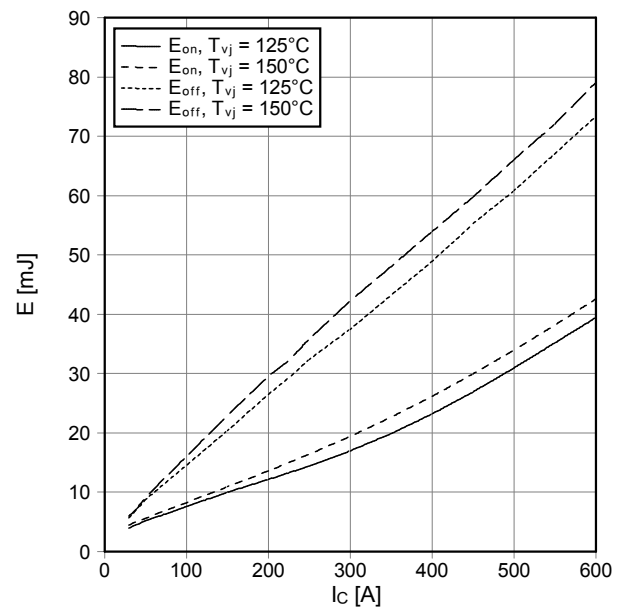
Schaltverluste IGBT-Wechselr. (typisch) switching losses IGBT-inverter (typical) E_{on} = f(I_c) , E_{off} = f(I_c) V_{GE} = \pm 15\text{ V} , R_{Gon} = 1.3\ \Omega , R_{Goff} = 1.3\ \Omega , V_{CE} = 600\text{ V}
