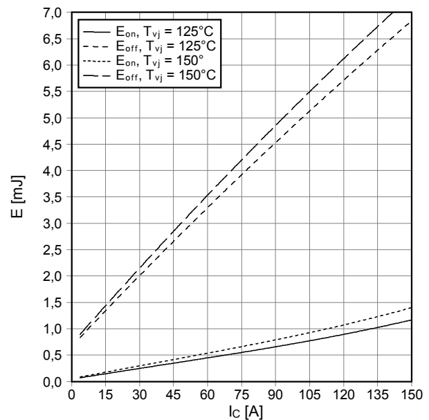
Schaltverluste IGBT-Wechselr. (typisch) switching losses IGBT-inverter (typical) E_{on} = f(I_c) , E_{off} = f(I_c) V_{GE} = \pm 15\text{ V} , R_{Gon} = 5.1\ \Omega , R_{Goff} = 5.1\ \Omega , V_{CE} = 300\text{ V}
