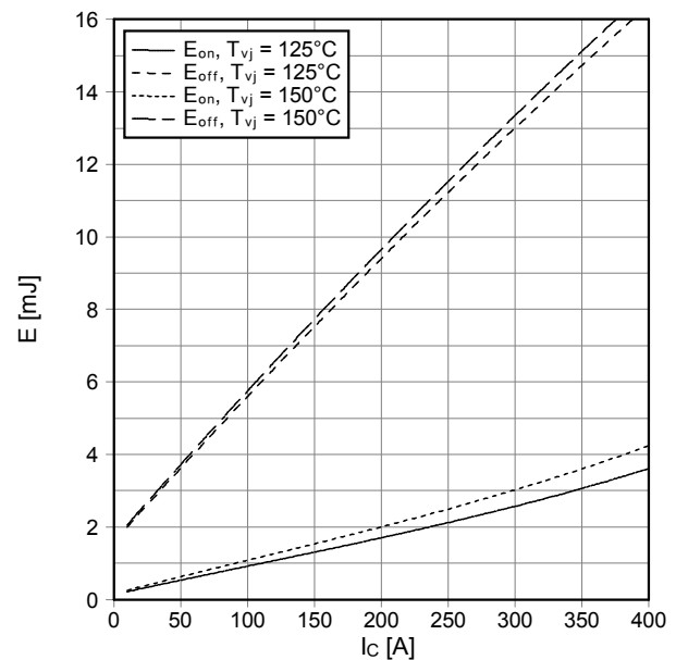
Schaltverluste IGBT-Wechselr. (typisch) switching losses IGBT-inverter (typical) E_{on} = f(I_c) , E_{off} = f(I_c) V_{GE} = \pm 15\text{ V} , R_{Gon} = 2\ \Omega , R_{Goff} = 2\ \Omega , V_{CE} = 300\text{ V}
