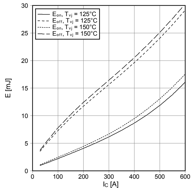
Schaltverluste IGBT-Wechselr. (typisch) switching losses IGBT-inverter (typical) E_{on} = f(I_c) , E_{off} = f(I_c) V_{GE} = \pm 15\text{ V} , R_{Gon} = 2.2\ \Omega , R_{Goff} = 1.5\ \Omega , V_{CE} = 300\text{ V}
