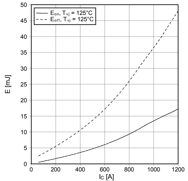
Schaltverluste IGBT-Brems-Chopper switching losses IGBT-brake-chopper E_{on} = f(I_c) , E_{off} = f(I_c) V_{GE} = \pm 15\text{ V} , R_{Gon} = 2.4\ \Omega , R_{Goff} = 2.4\ \Omega , V_{CE} = 150\text{ V}
