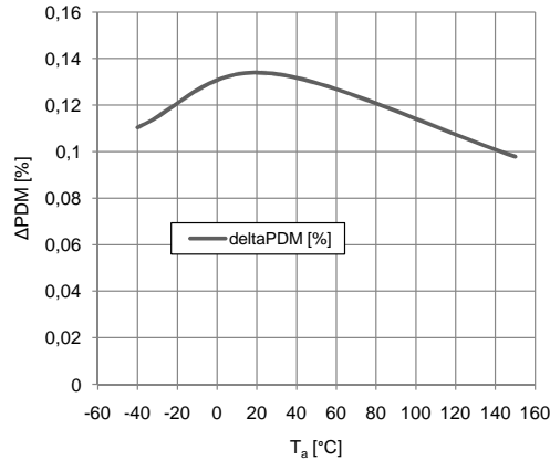
DC-Offset \Sigma/\Delta -Wandler (typisch) dc offset \Sigma/\Delta converter (typical) \Delta PDM = f(T_a) V_{CC1} = 5V
