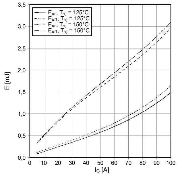
Schaltverluste IGBT-Wechselr. (typisch) switching losses IGBT-inverter (typical) E_{on} = f(I_c) , E_{off} = f(I_c) V_{GE} = \pm 15\text{ V} , R_{Gon} = 6.8\ \Omega , R_{Goff} = 6.8\ \Omega , V_{CE} = 300\text{ V}
