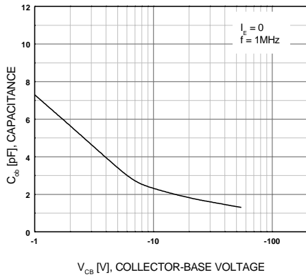
Figure 3. Output Capacitance
