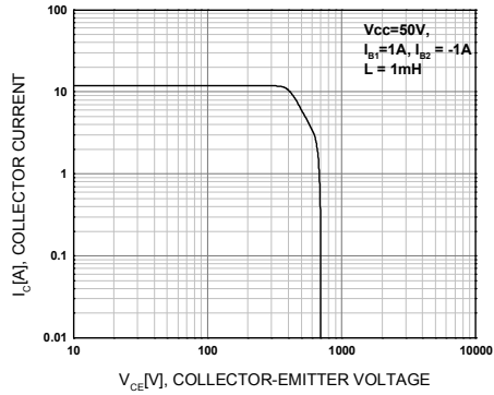
Figure 7. Reverse Bias Safe Operating Area
