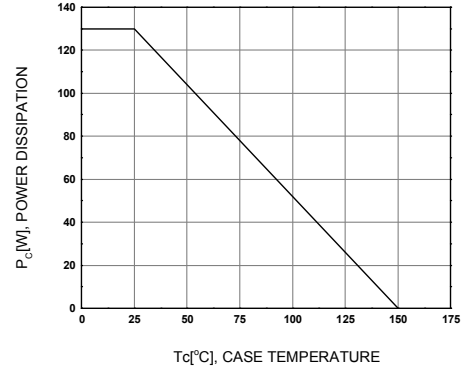
Figure 8. Power Derating
