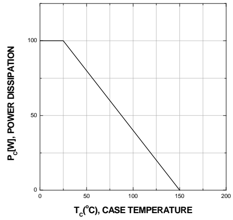
Figure 17. Power Derating
