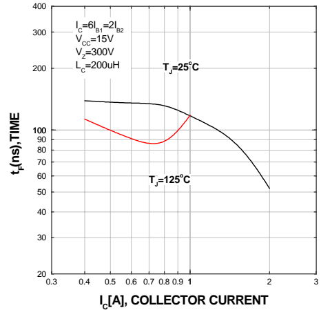
Figure 13. Inductive Switching Time, t_f
