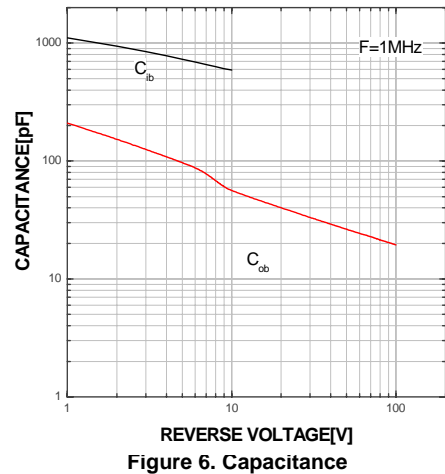
Figure 6. Capacitance
