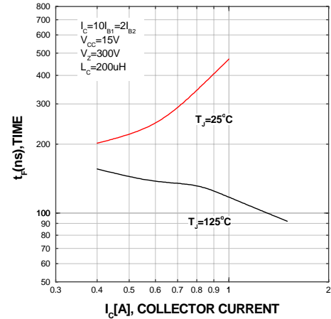
Figure 14. Inductive Switching Time, t_f
