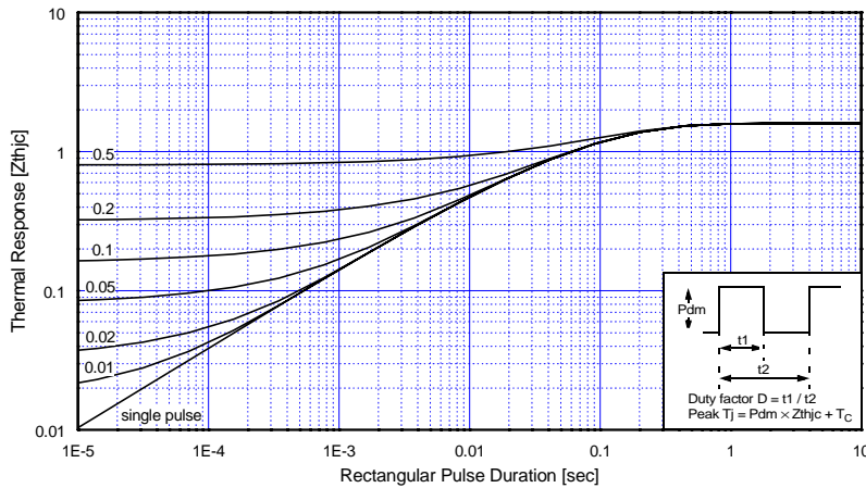
Fig 17. Transient Thermal Impedance of IGBT
