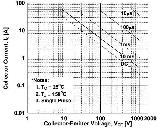
Figure 10. SOA Characteristics
