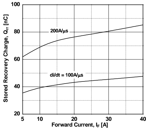
Figure 21. Stored Charge
