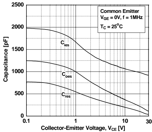
Figure 9. Capacitance Characteristics
