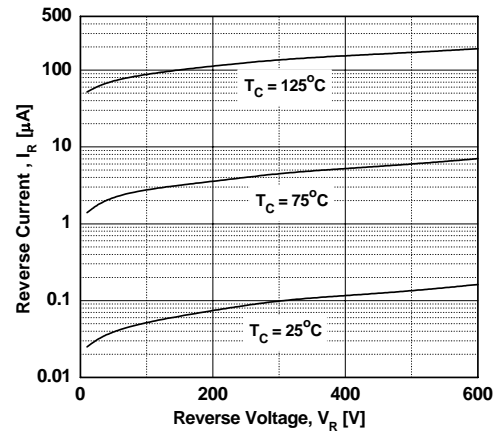
Figure 20. Reverse Current
