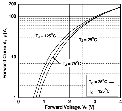
Figure 19. Forward Characteristics
