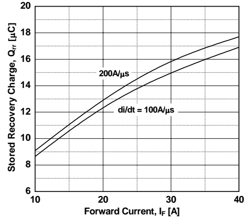
Figure 20. Stored Charge
