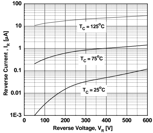
Figure 20. Reverse Current
