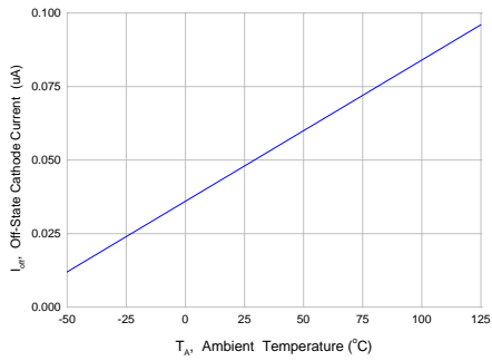
Figure 6. OFF-State Cathode Current vs. Ambient Temperature
