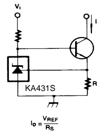
Figure 17. Constant-Current Sink
