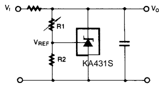
Figure 13. Shunt Regulator
