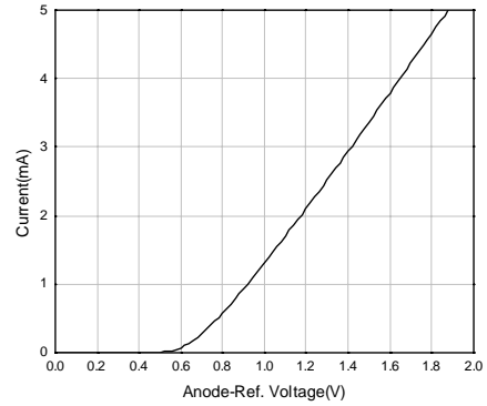
Figure 11. Anode-Reference Diode Curve
