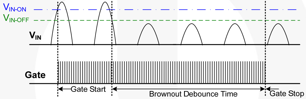
Figure 6. Brownout Behavior
