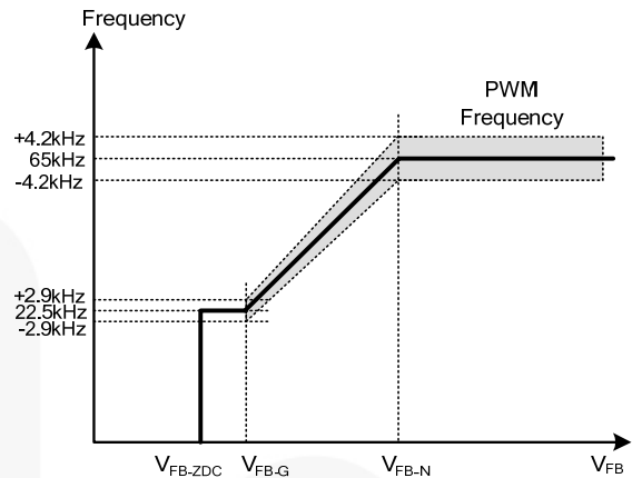
Figure 25. PWM Frequency
