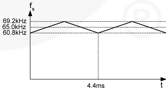
Figure 27. Frequency Hopping
