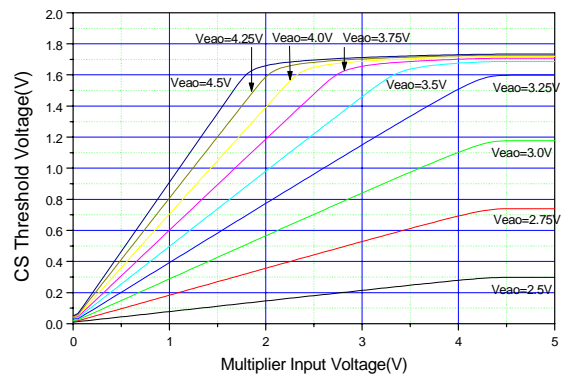
Figure 2. Multiplier Input Voltage vs Current Sensing Threshold
