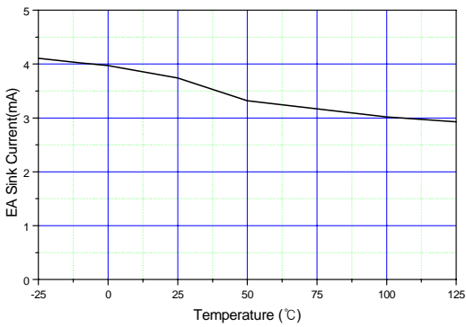
Figure 9. Error Amplifier Sink Current vs Temperature
