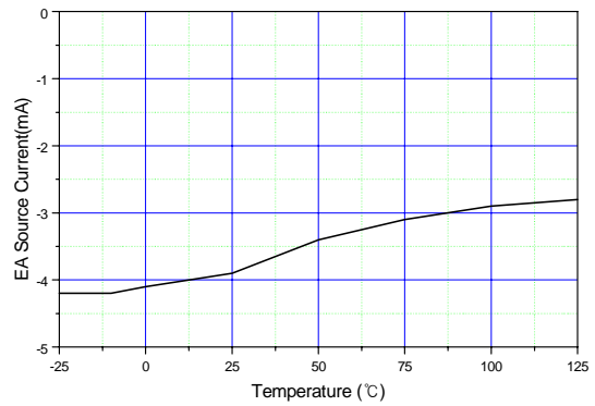
Figure 8. Error Amplifier Source Current vs Temperature
