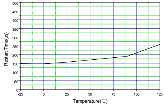
Figure 14. Restart Time vs Temperature
