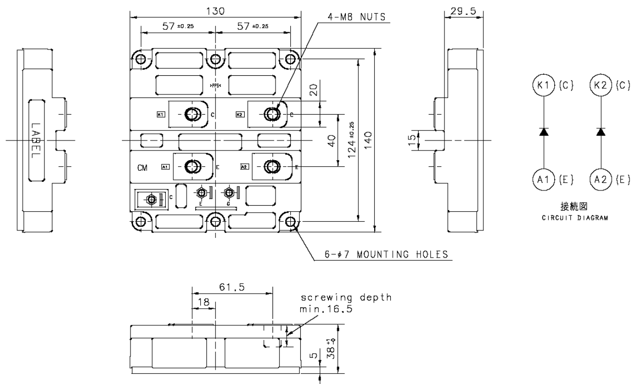
Fig. 1 - Outline drawing
