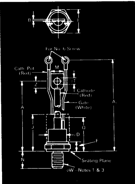
Conforms to TO-94 Outline
