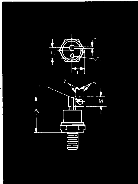
Conforms to TO-83 Outline
