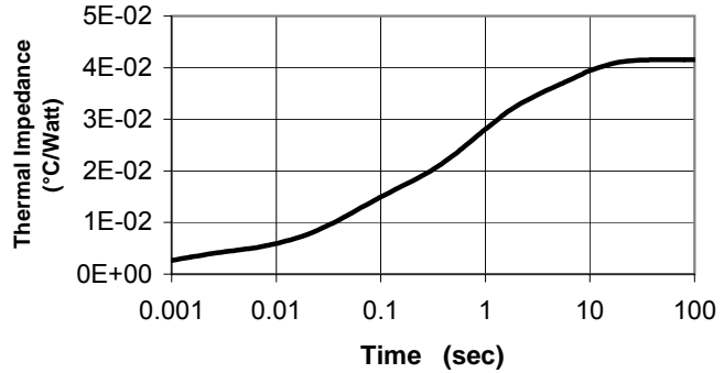
MAXIMUM TRANSIENT THERMAL IMPEDANCE
