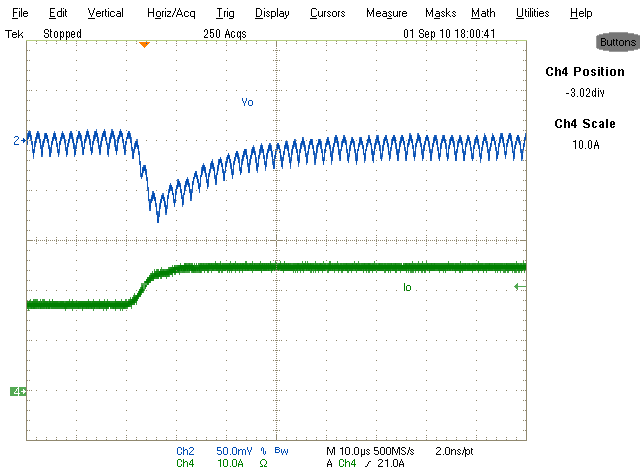
Fig. 9: Transient Response, 17.5A to 25A step (2.5A/us) Ch 2 :V out , Ch 4 : Io
