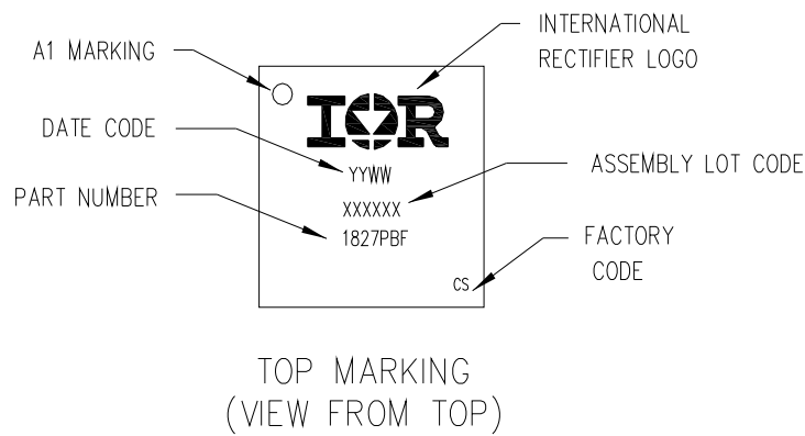
Fig. 19. Part Marking
