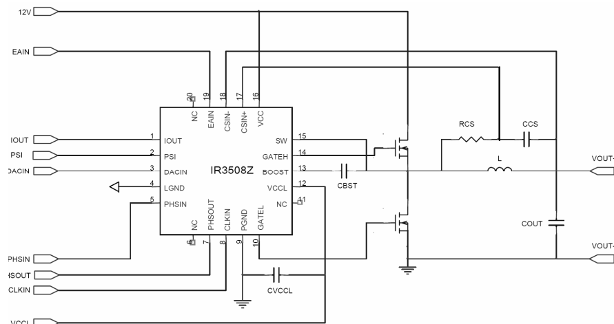
Figure 1 Application Circuit
