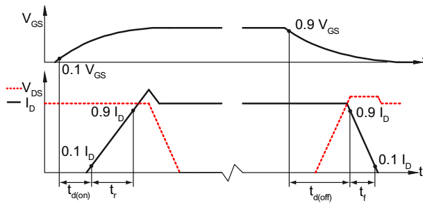
Fig. 20 Definition of switching times
