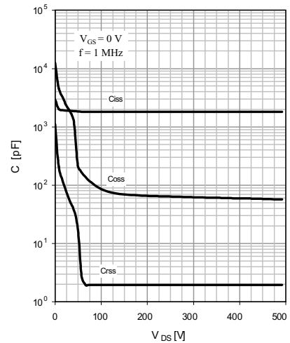
Fig. 9 Typ. capacitances
