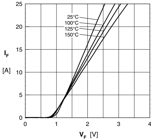
Fig. 12 Forward characteristic of boost diode
