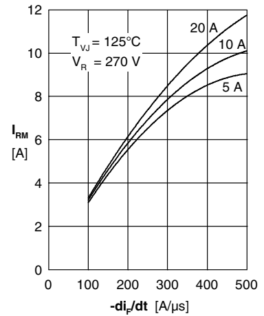
Fig. 3 Typ. reverse recovery current I_{RM} versus -di_F/dt
