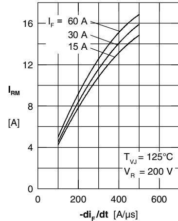
Fig. 3 Typ. reverse recovery current I_{RM} versus -di_F/dt
