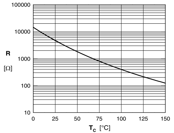
Fig. 10 Typ. NTC resistance vs. temperature
