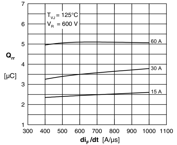
Fig. 8 Typ. reverse recov.charge Q_{rr} vs. di/dt
