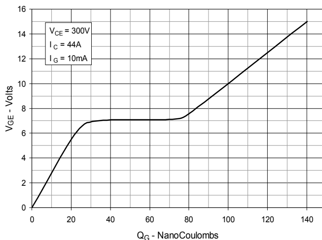
Fig. 8. Gate Charge
