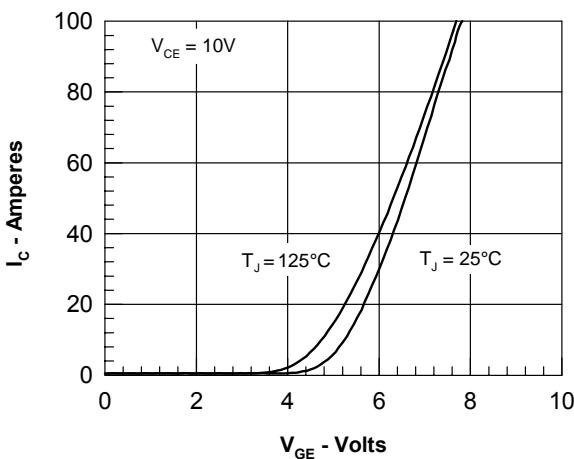
Figure 5. Admittance Curves
